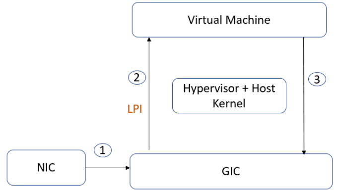
Fig. 7: NIC delivers interrupt in the form of LPI
