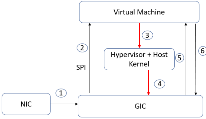
Fig. 6: NIC delivers interrupt in the form of SPI
