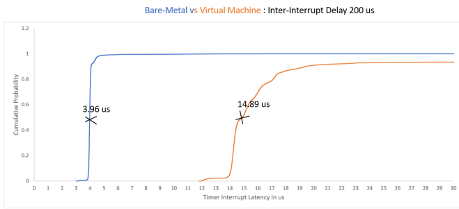
Fig. 11: Kernel Level Timer Interrupt Latency Test values plotted against Cumulative Probability
