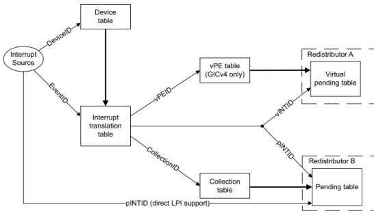
Fig. 4: Physical and Virtual LPI Delivery Flow
