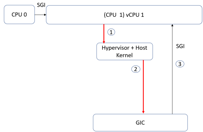
Fig. 10: SGI delivery between two pCPU and vCPU
