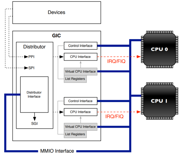
Fig. 2: Generic Interrupt Controller with Virtualization hardware support
