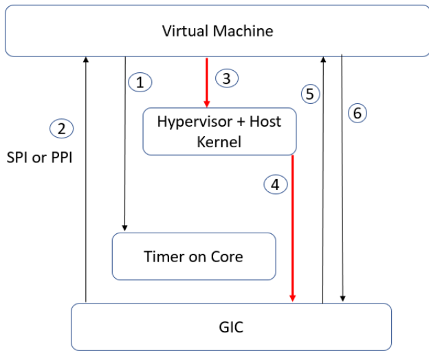
Fig. 8: Timer Interrupt delivered as SPl or PPI
