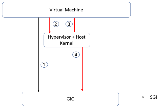
Fig. 9: SGI delivery between two vCPU
