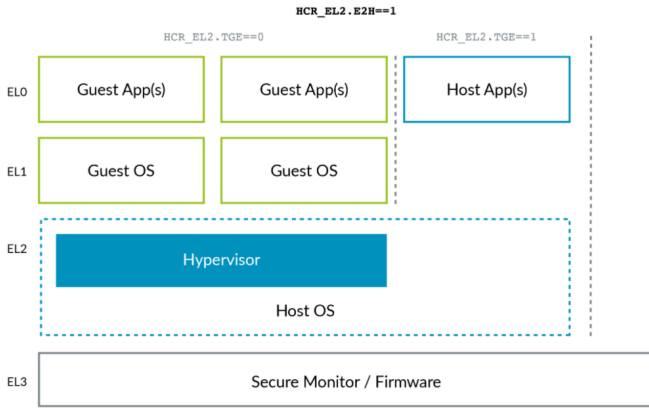
Fig. 3: Host Kernel runs along with Hypervisor in EL2 with VHE support
