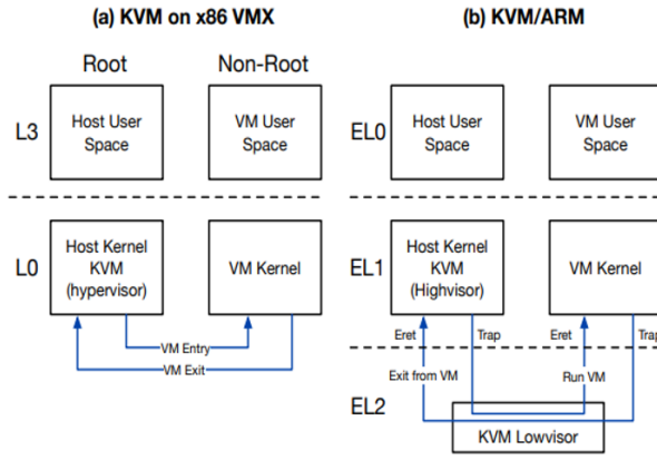
Fig. 1: Exception Levels x86 VS ARM
