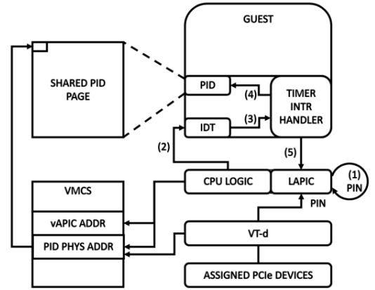
Fig. 5: Delivering Timer interrupt and IPI directly with VT-d
